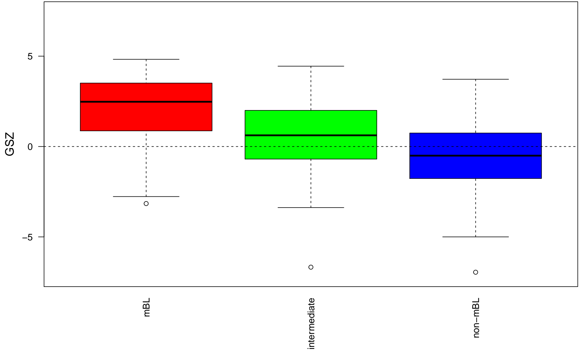
Tirosh_top50 correlated genes PC1
