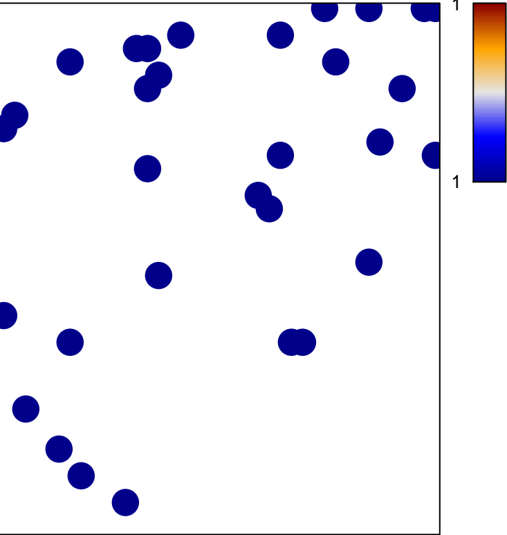
# features = 31
